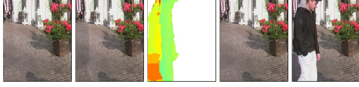
Fig. 5. Gradient-domain fusion. Left to right: previous frame (inpainted, blended) aligned using optical flow; current frame (inpainted); color-coded labeling of the inpainting sources; resulting gradient-domain fusion; original current frame for reference.
